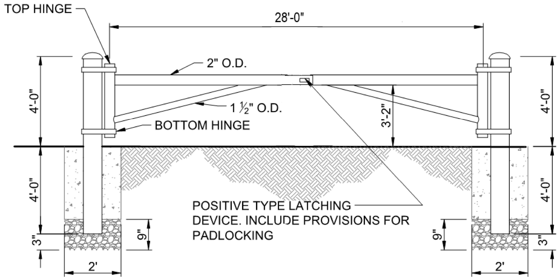
DOUBLE METAL SWING ARM GATE NOT TO SCALE
